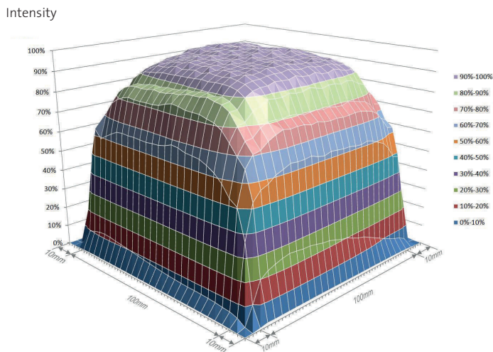
Intensity distribution LED Spot 100, distance 5 mm
