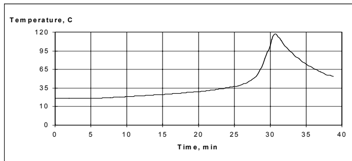
Typical Exotherm Curve for MA422 at 23°C (10 grams) 5
